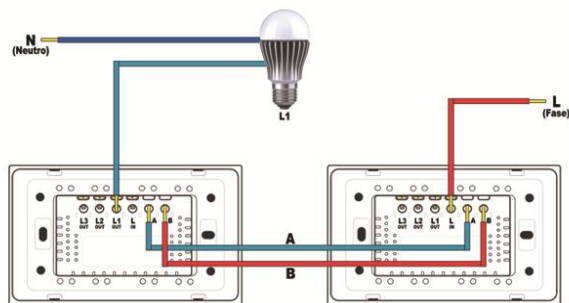
VL-C301S-81, VL-C301S-82
